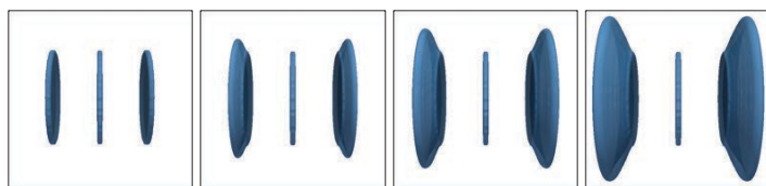
Figure 1. Growth of three parallel penny-shaped fractures in 3D using the active set method. The middle fracture growth is shunned by stress shadowing effect similar to those studied in 2D fracture growth (ICES Report 14-20).
